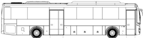
Layout 12 m : 55 passengers seats
